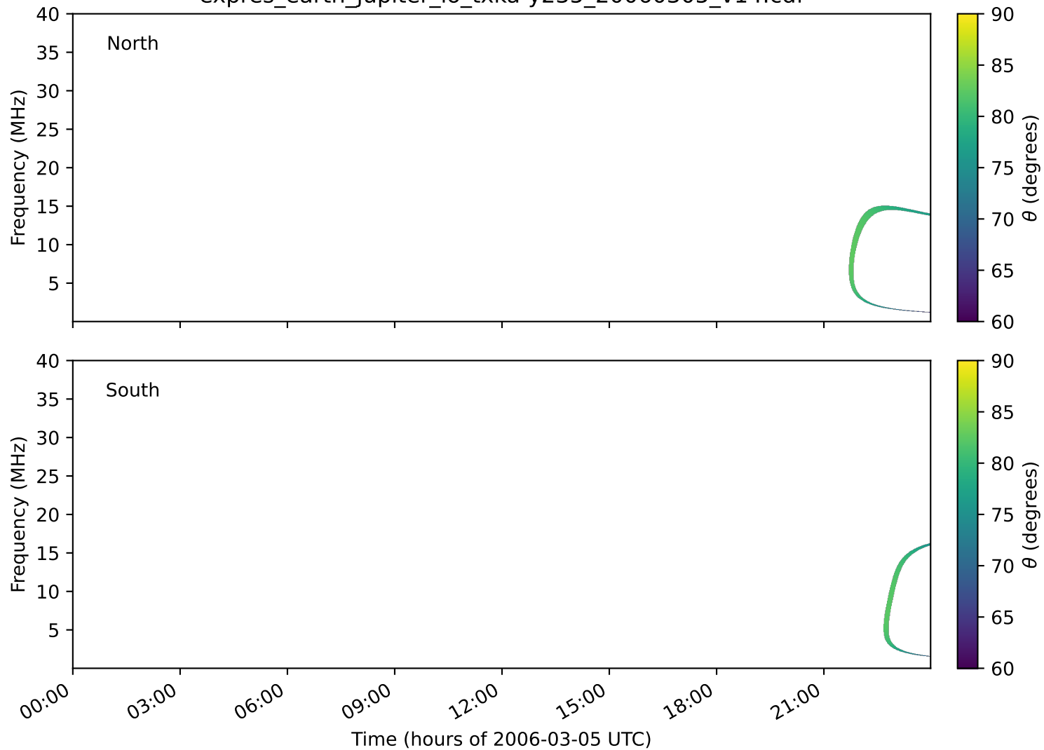
expres_earth_jupiter_io_txka-y235_20060305_v14.cdf
