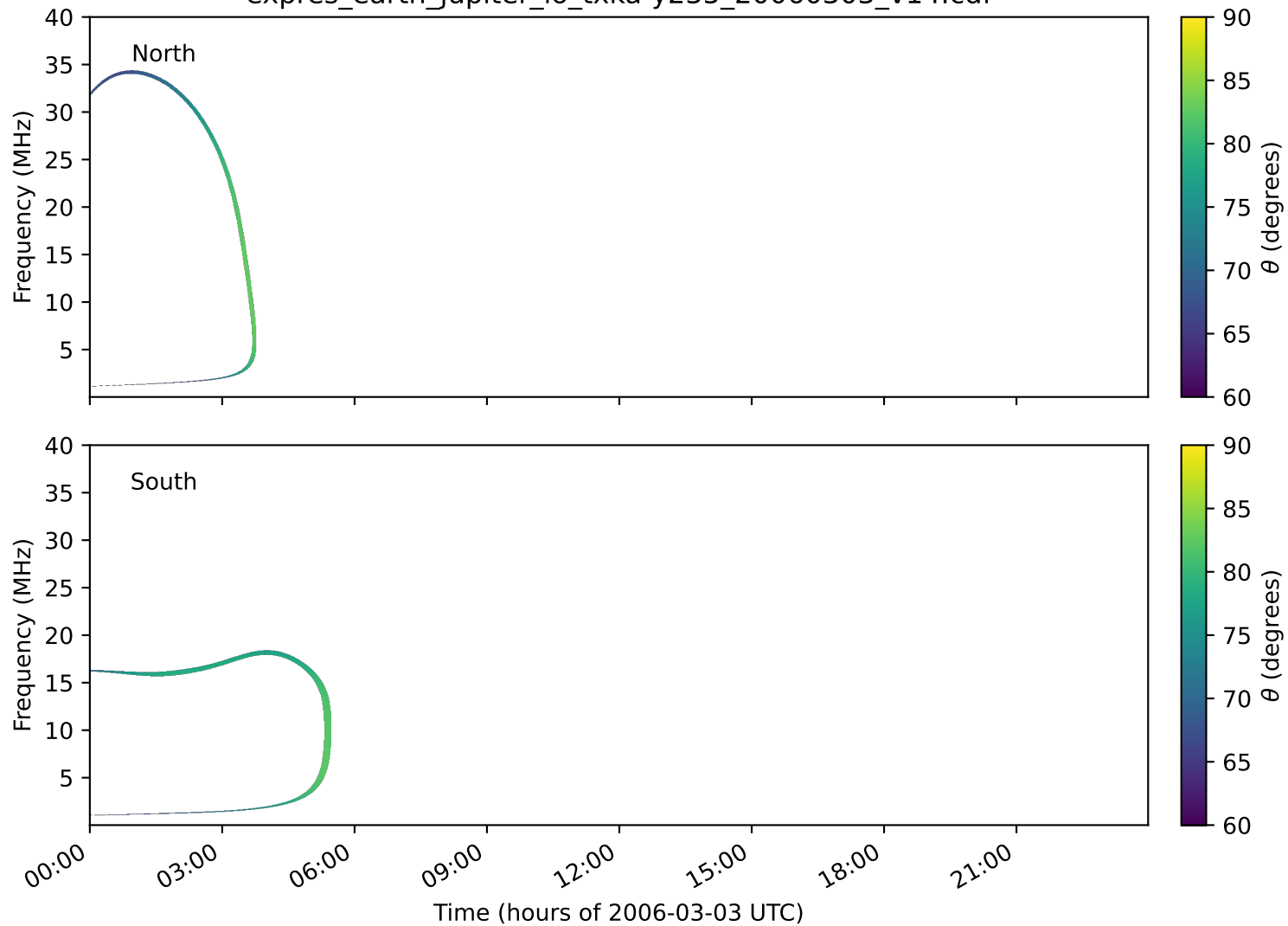
expres_earth_jupiter_io_txka-y235_20060303_v14.cdf
