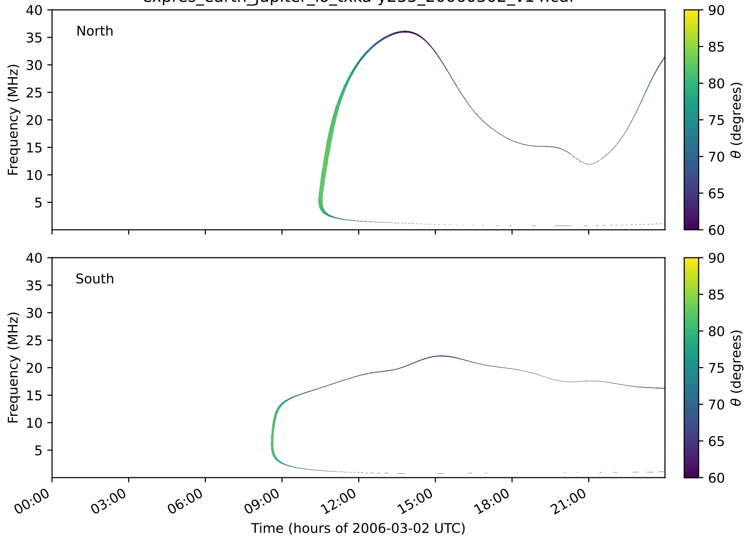
expres_earth_jupiter_io_txka-y235_20060302_v14.cdf
