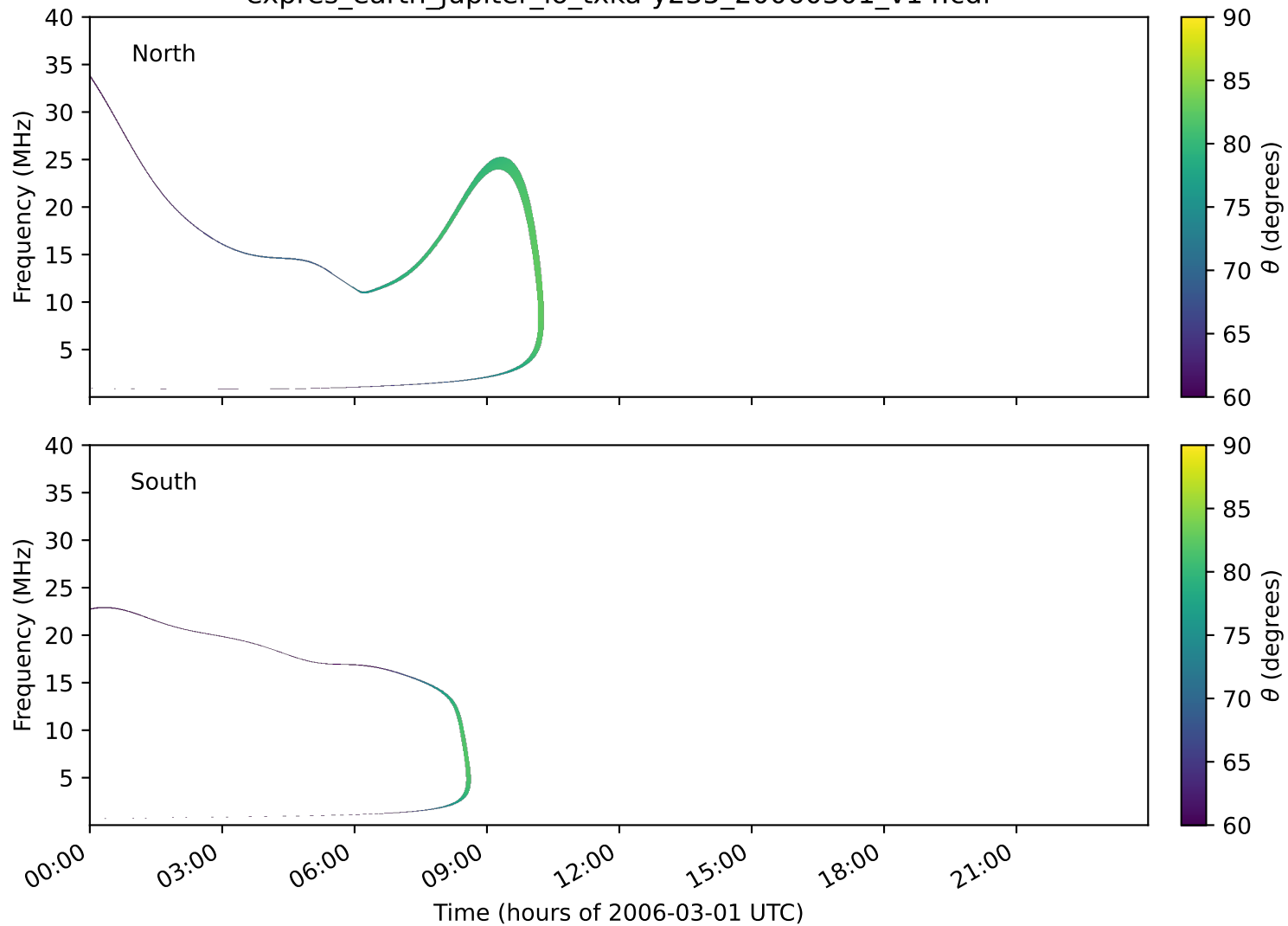
expres_earth_jupiter_io_txka-y235_20060301_v14.cdf
