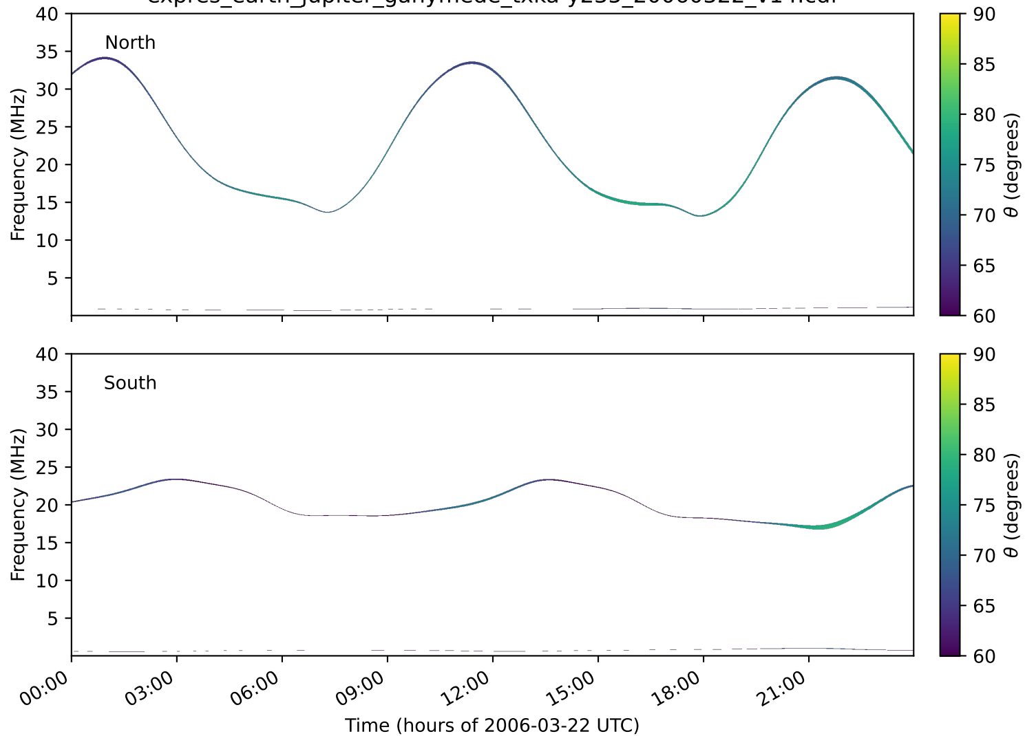
expres_earth_jupiter_ganymede_txka-y235_20060322_v14.cdf
