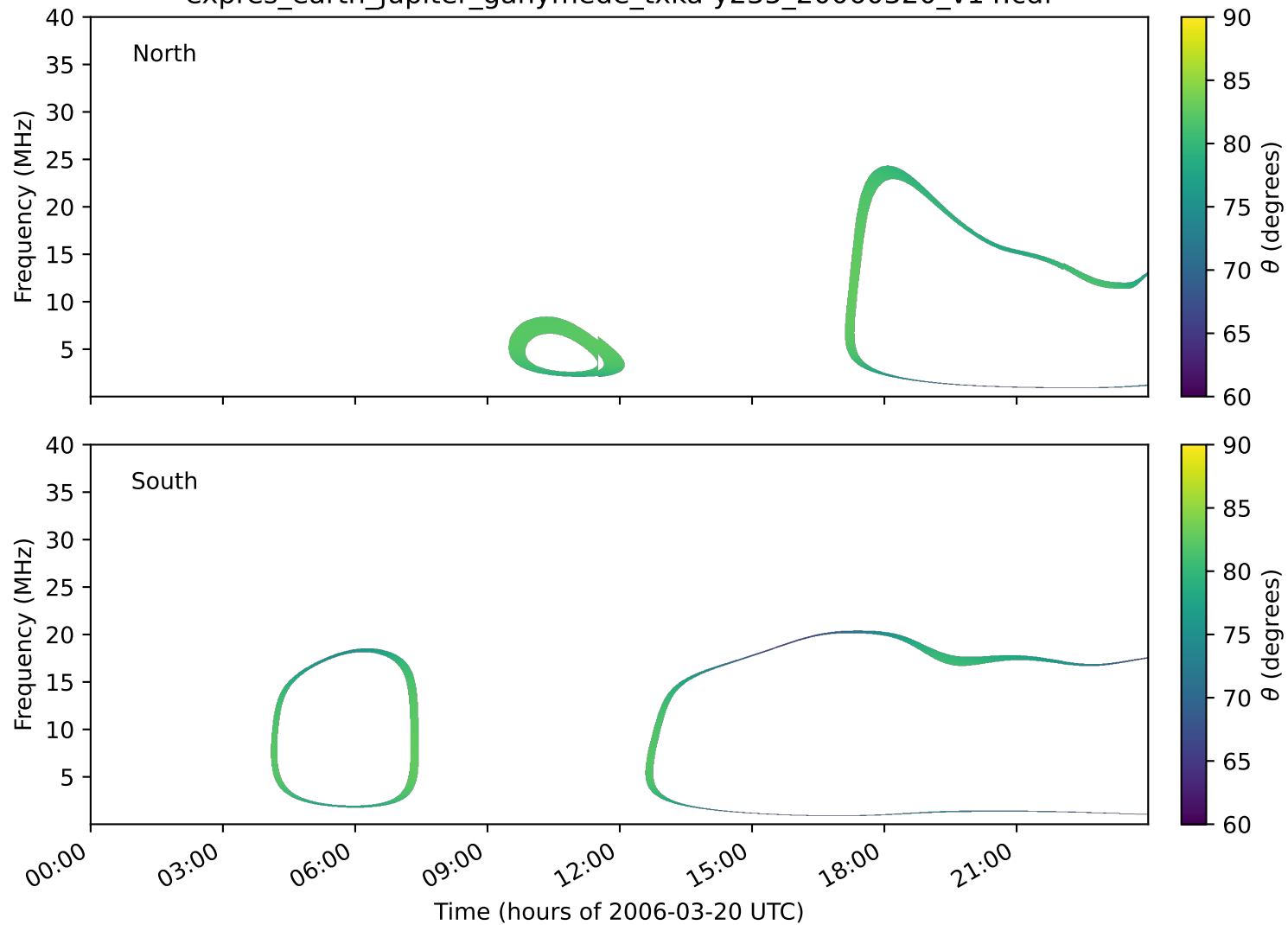
expres_earth_jupiter_ganymede_txka-y235_20060320_v14.cdf
