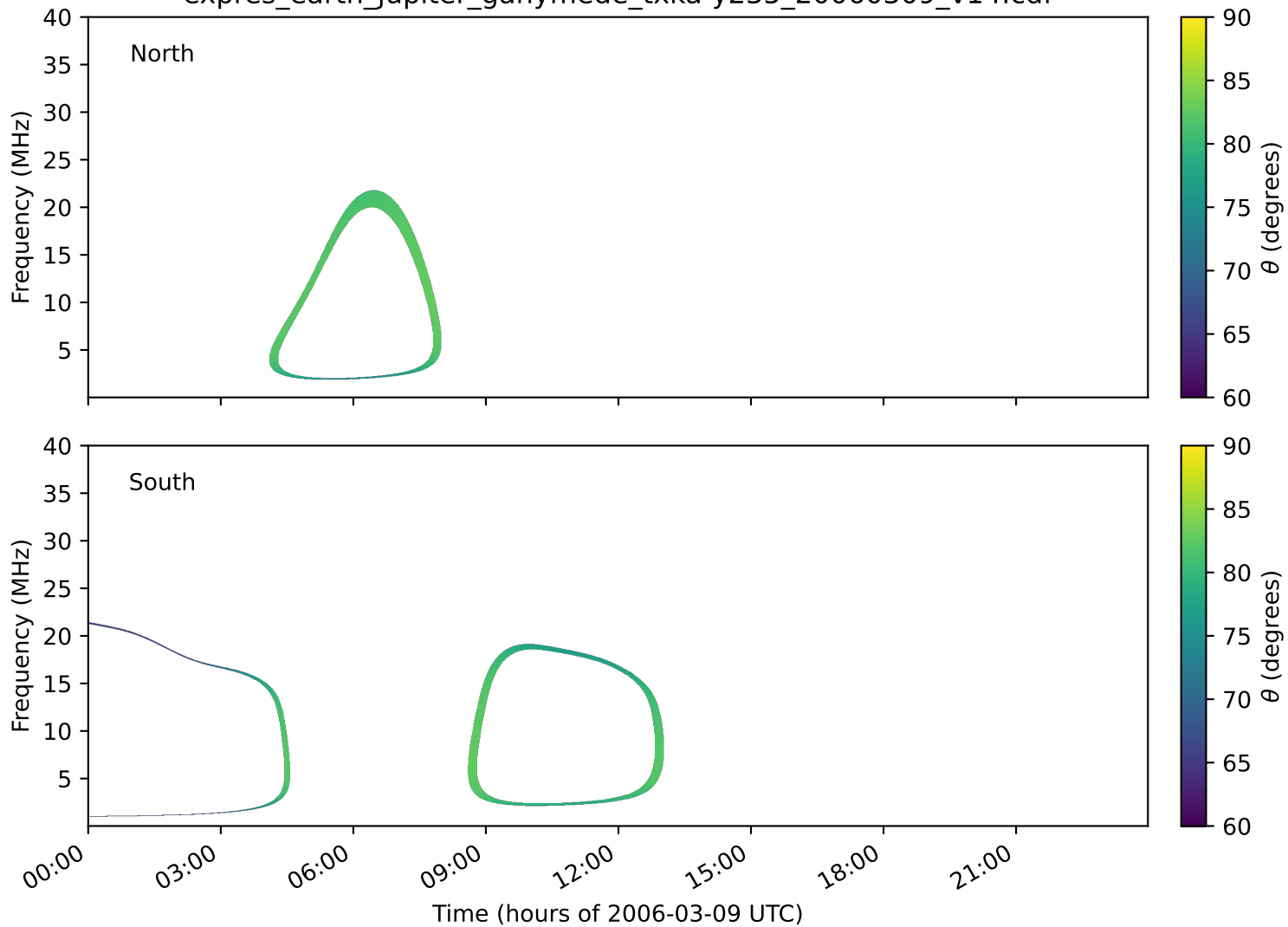
expres_earth_jupiter_ganymede_txka-y235_20060309_v14.cdf
