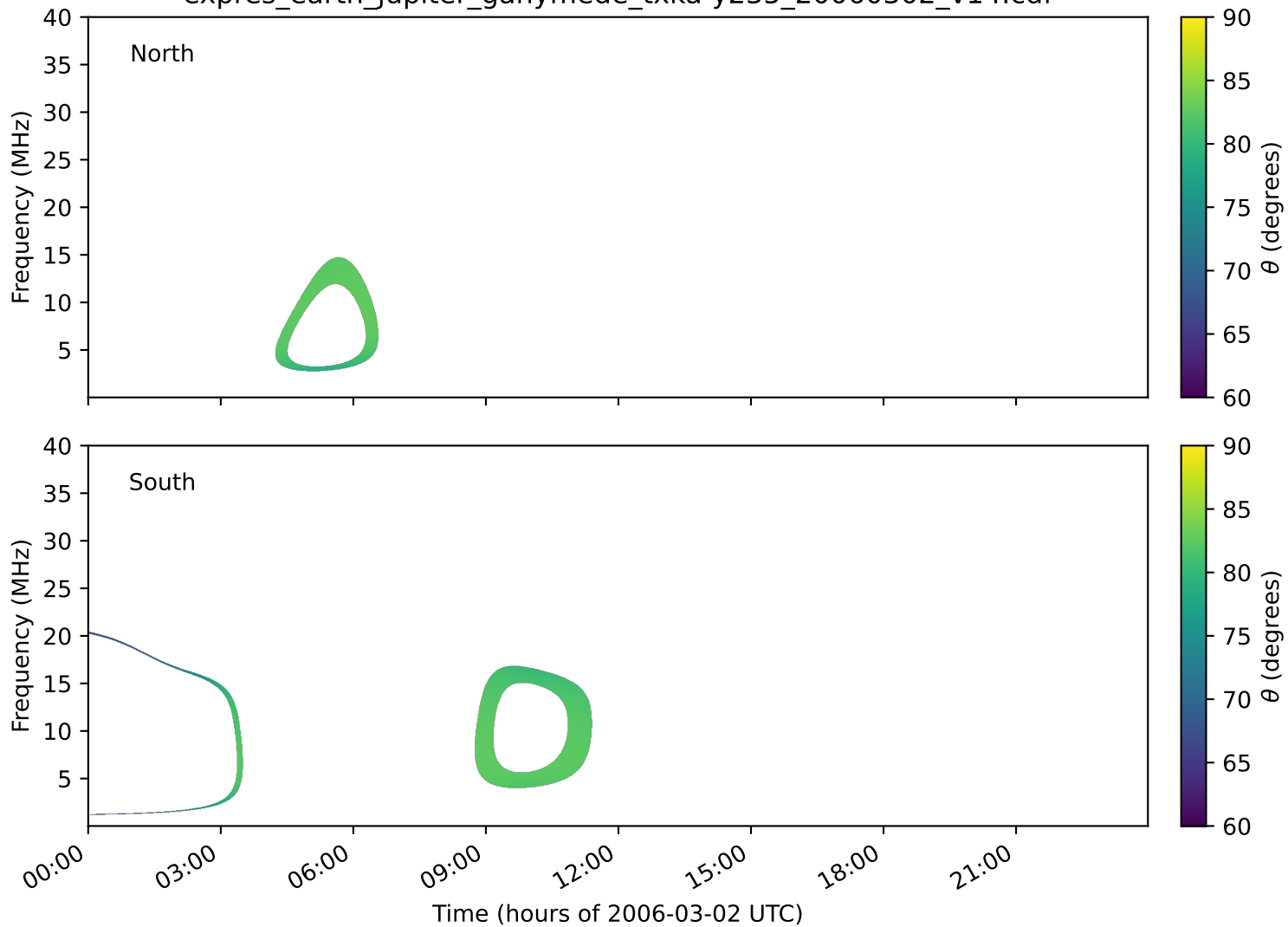
expres_earth_jupiter_ganymede_txka-y235_20060302_v14.cdf
