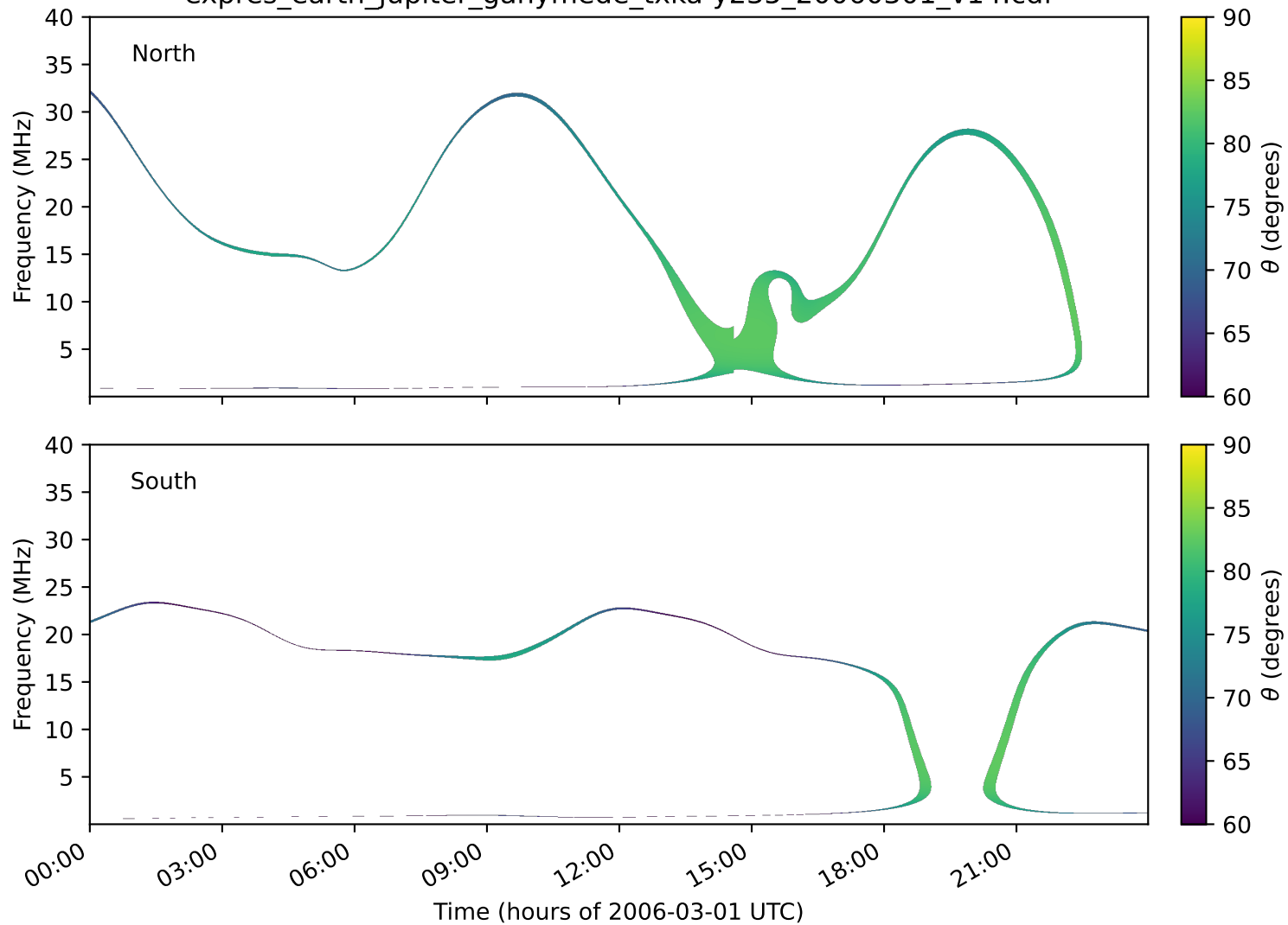
expres_earth_jupiter_ganymede_txka-y235_20060301_v14.cdf
