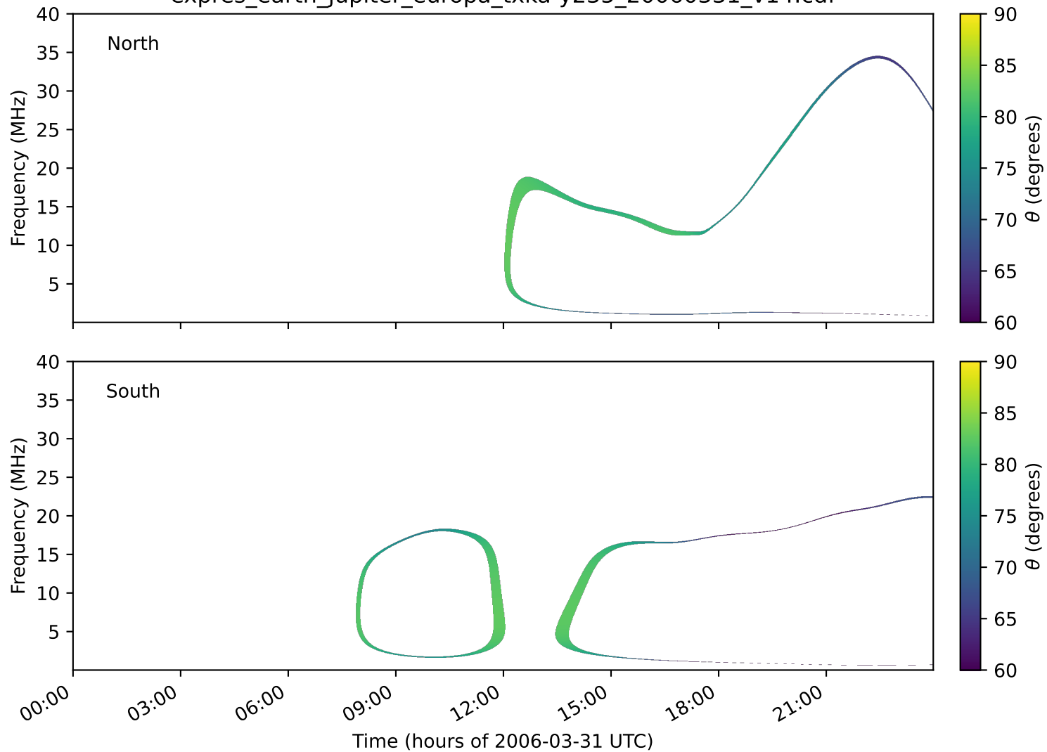
expres_earth_jupiter_europa_txka-y235_20060331_v14.cdf
