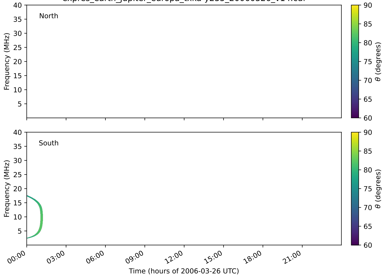
expres_earth_jupiter_europa_txka-y235_20060326_v14.cdf
