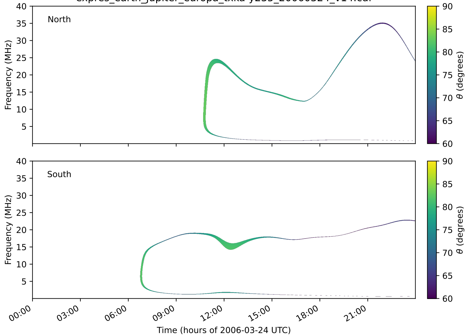
expres_earth_jupiter_europa_txka-y235_20060324_v14.cdf
