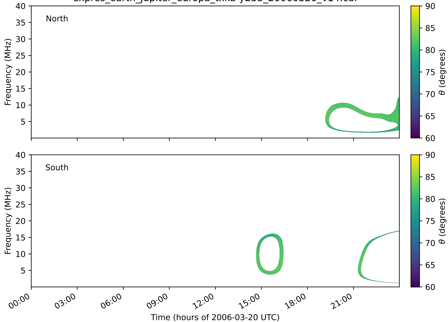
expres_earth_jupiter_europa_txka-y235_20060320_v14.cdf
