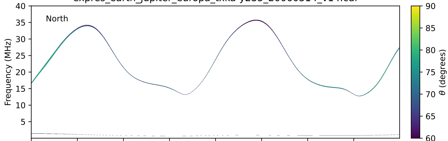
expres_earth_jupiter_europa_txka-y235_20060314_v14.cdf
