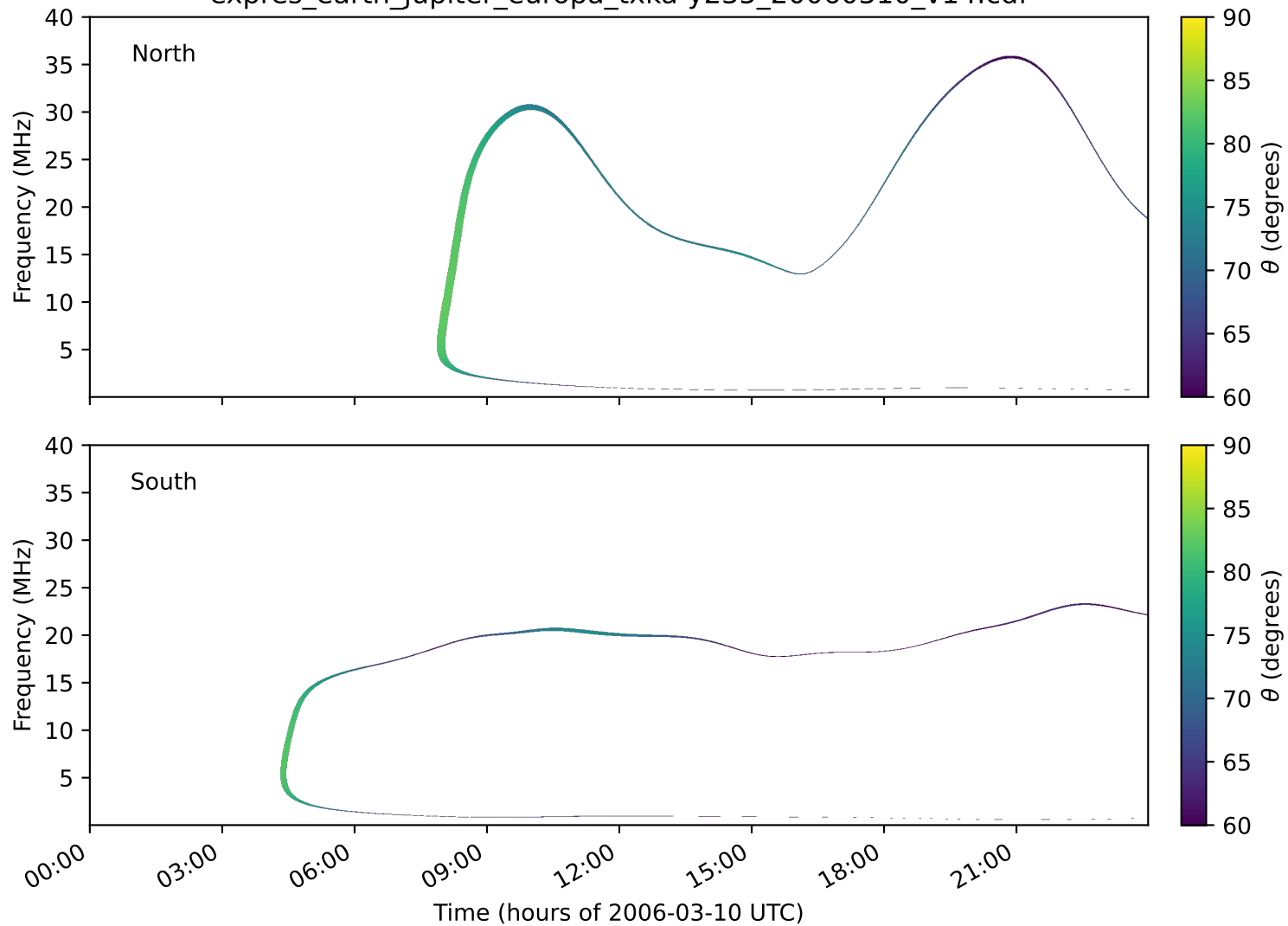
expres_earth_jupiter_europa_txka-y235_20060310_v14.cdf
