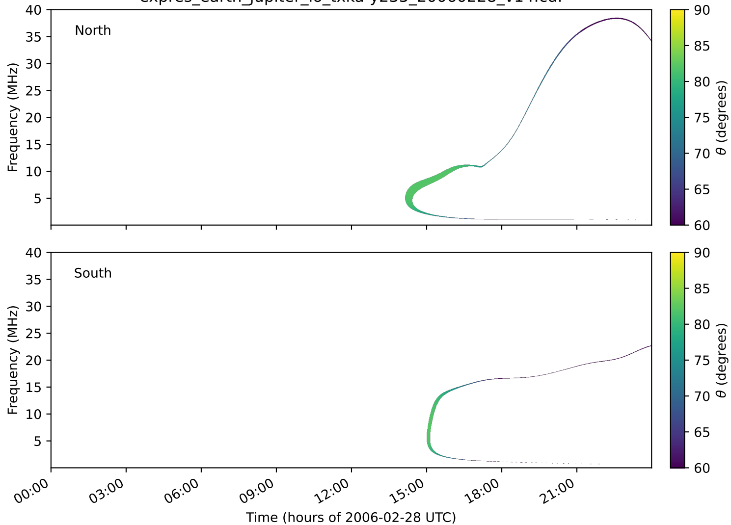
expres_earth_jupiter_io_txka-y235_20060228_v14.cdf
