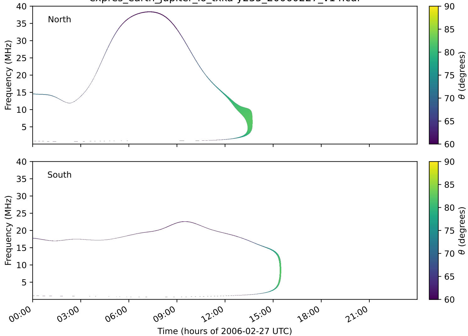
expres_earth_jupiter_io_txka-y235_20060227_v14.cdf
