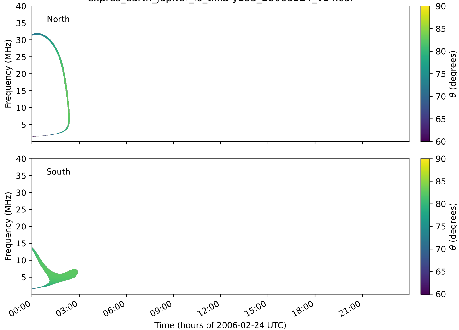
expres_earth_jupiter_io_txka-y235_20060224_v14.cdf
