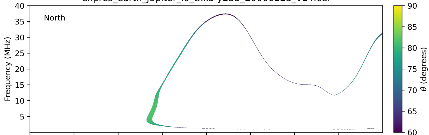
expres_earth_jupiter_io_txka-y235_20060223_v14.cdf
