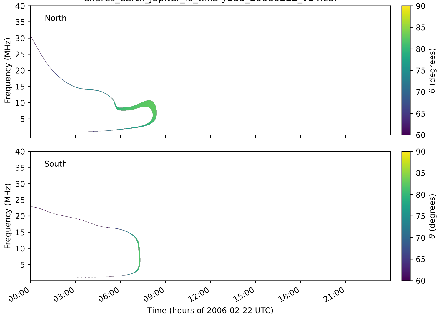
expres_earth_jupiter_io_txka-y235_20060222_v14.cdf
