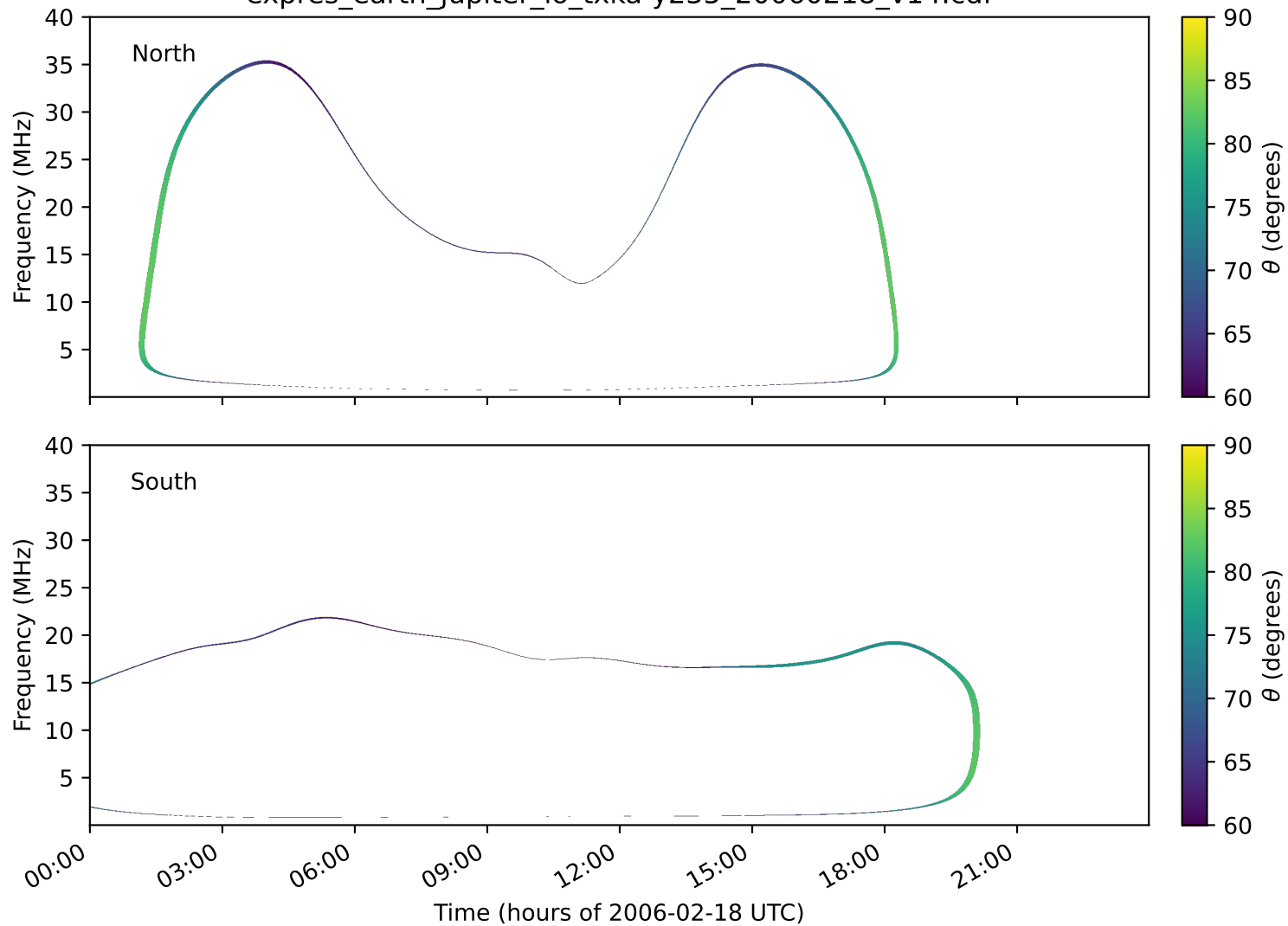
expres_earth_jupiter_io_txka-y235_20060218_v14.cdf
