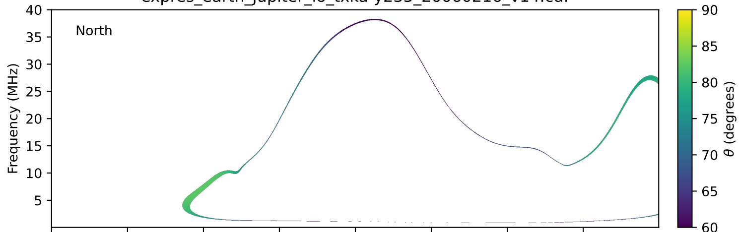
expres_earth_jupiter_io_txka-y235_20060216_v14.cdf
