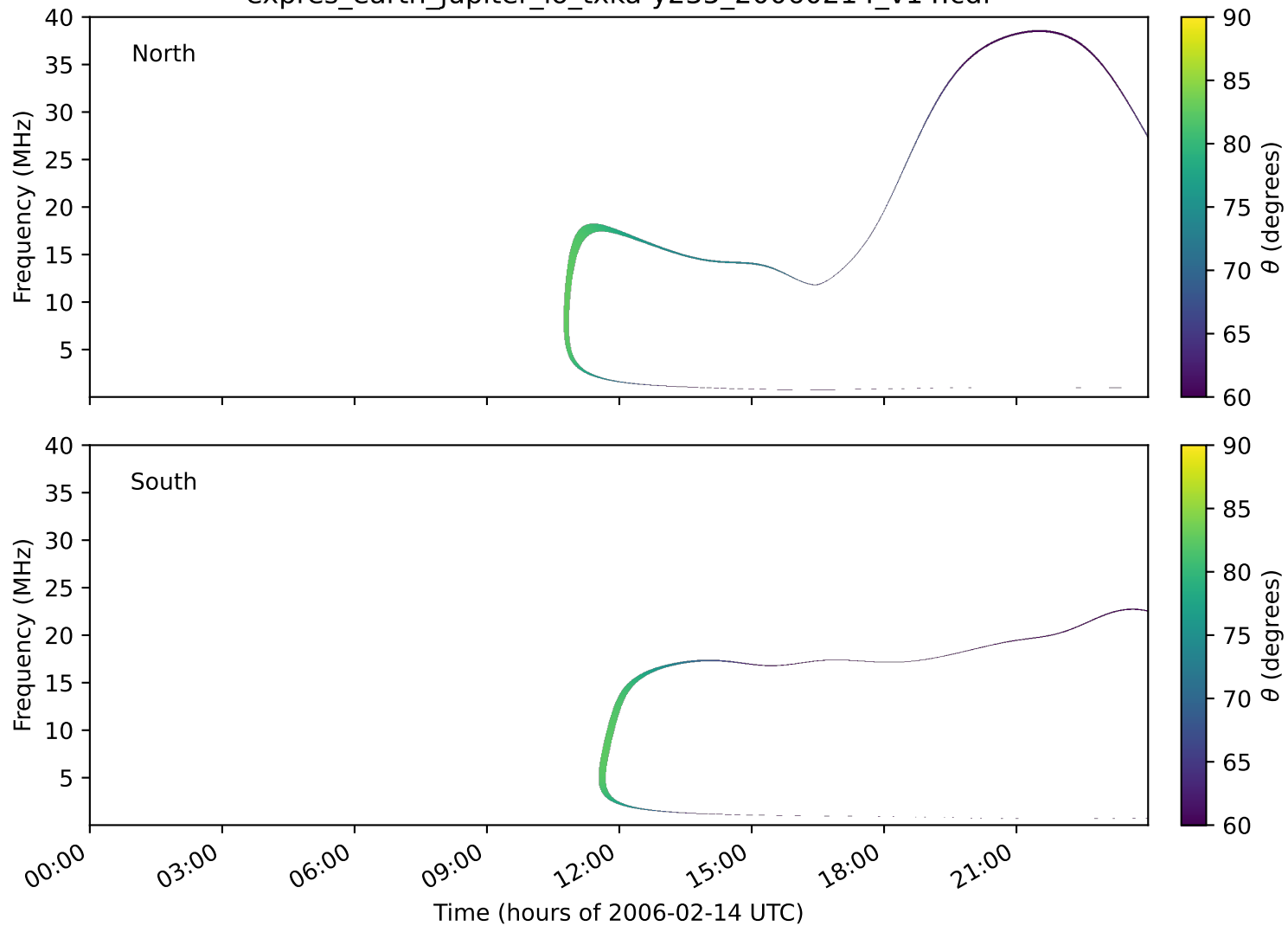
expres_earth_jupiter_io_txka-y235_20060214_v14.cdf
