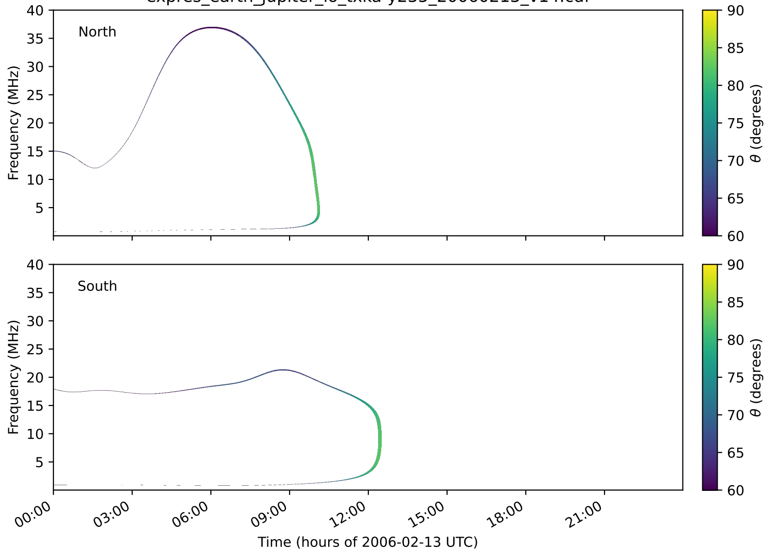
expres_earth_jupiter_io_txka-y235_20060213_v14.cdf
