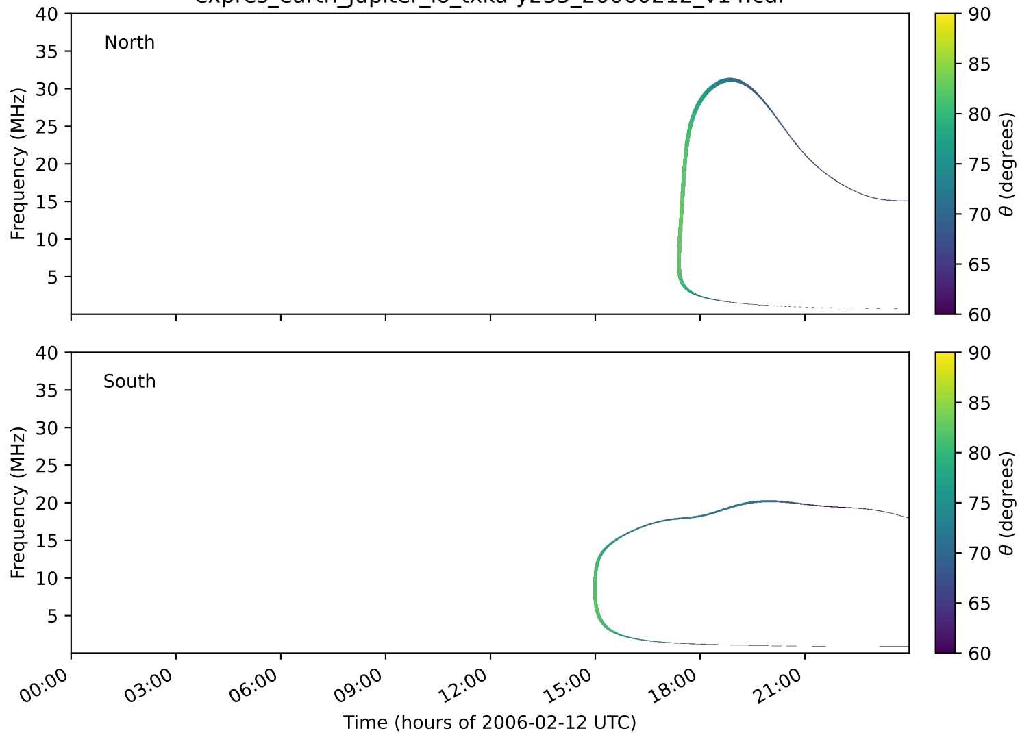
expres_earth_jupiter_io_txka-y235_20060212_v14.cdf
