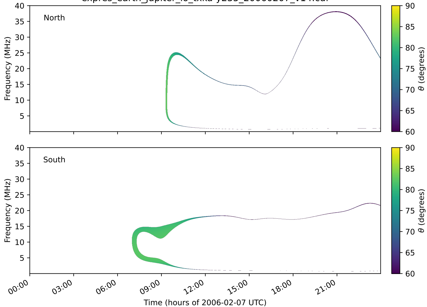
expres_earth_jupiter_io_txka-y235_20060207_v14.cdf
