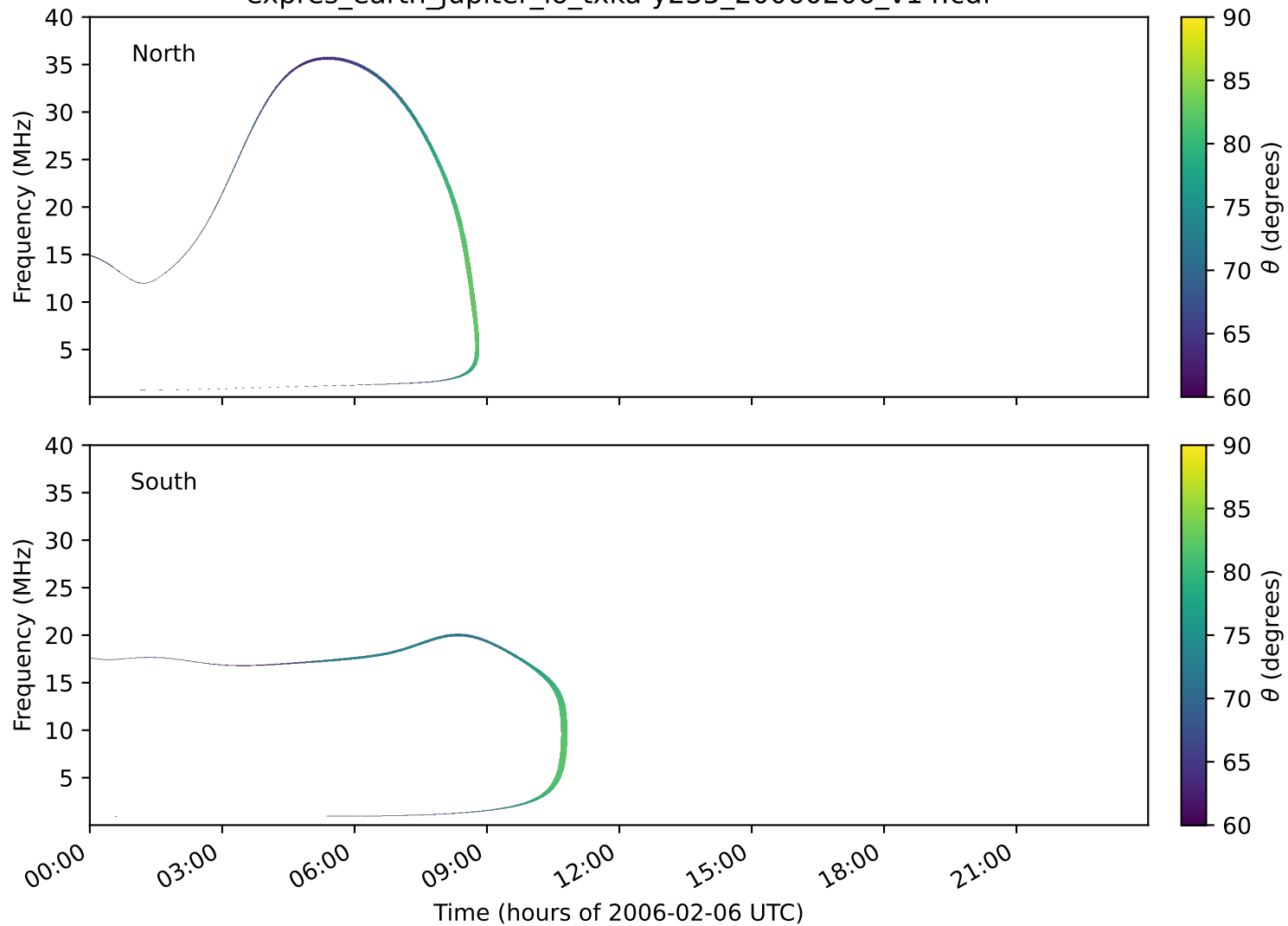
expres_earth_jupiter_io_txka-y235_20060206_v14.cdf
