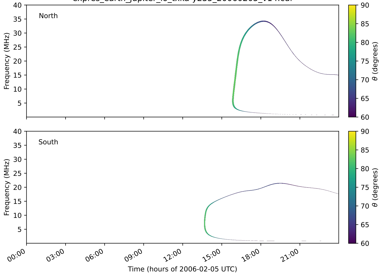
expres_earth_jupiter_io_txka-y235_20060205_v14.cdf
