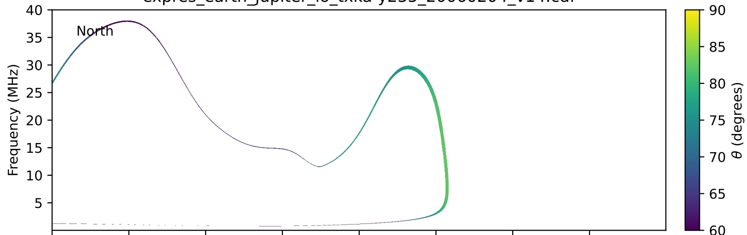
expres_earth_jupiter_io_txka-y235_20060204_v14.cdf
