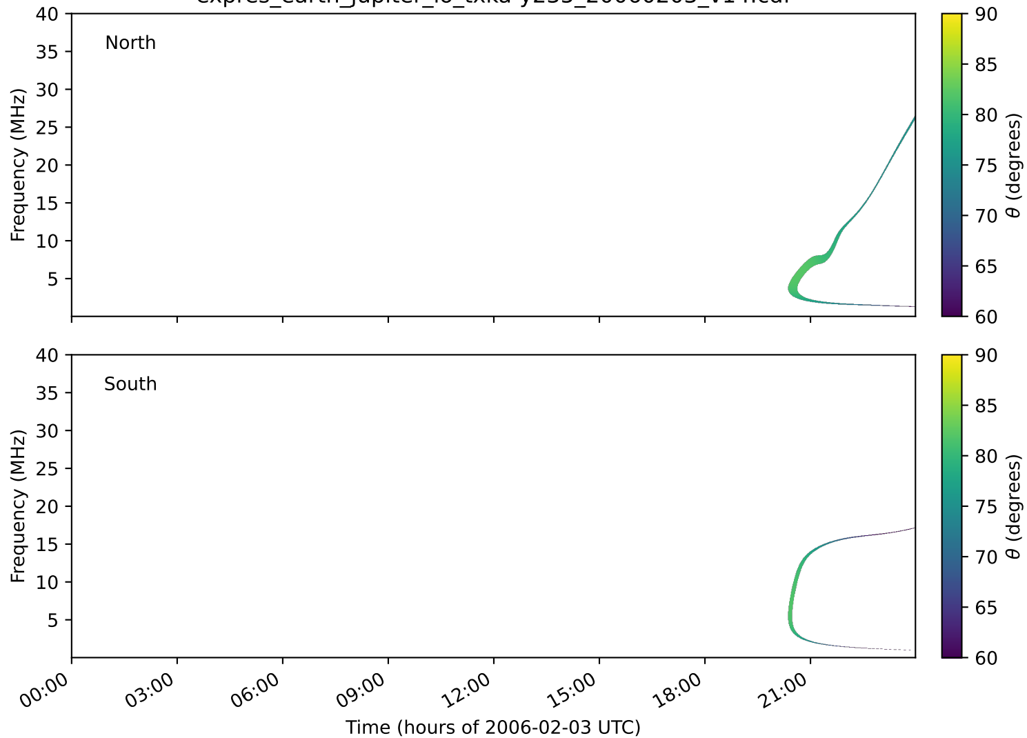
expres_earth_jupiter_io_txka-y235_20060203_v14.cdf
