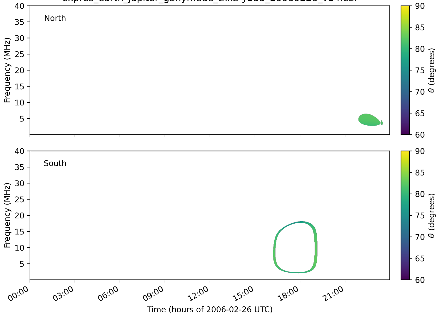
expres_earth_jupiter_ganymede_txka-y235_20060226_v14.cdf
