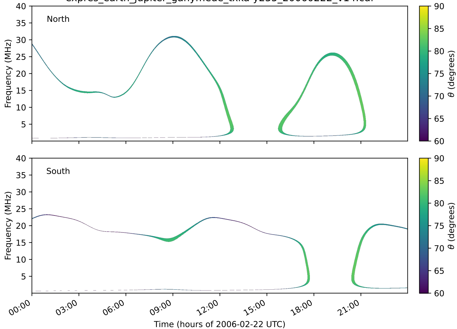
expres_earth_jupiter_ganymede_txka-y235_20060222_v14.cdf
