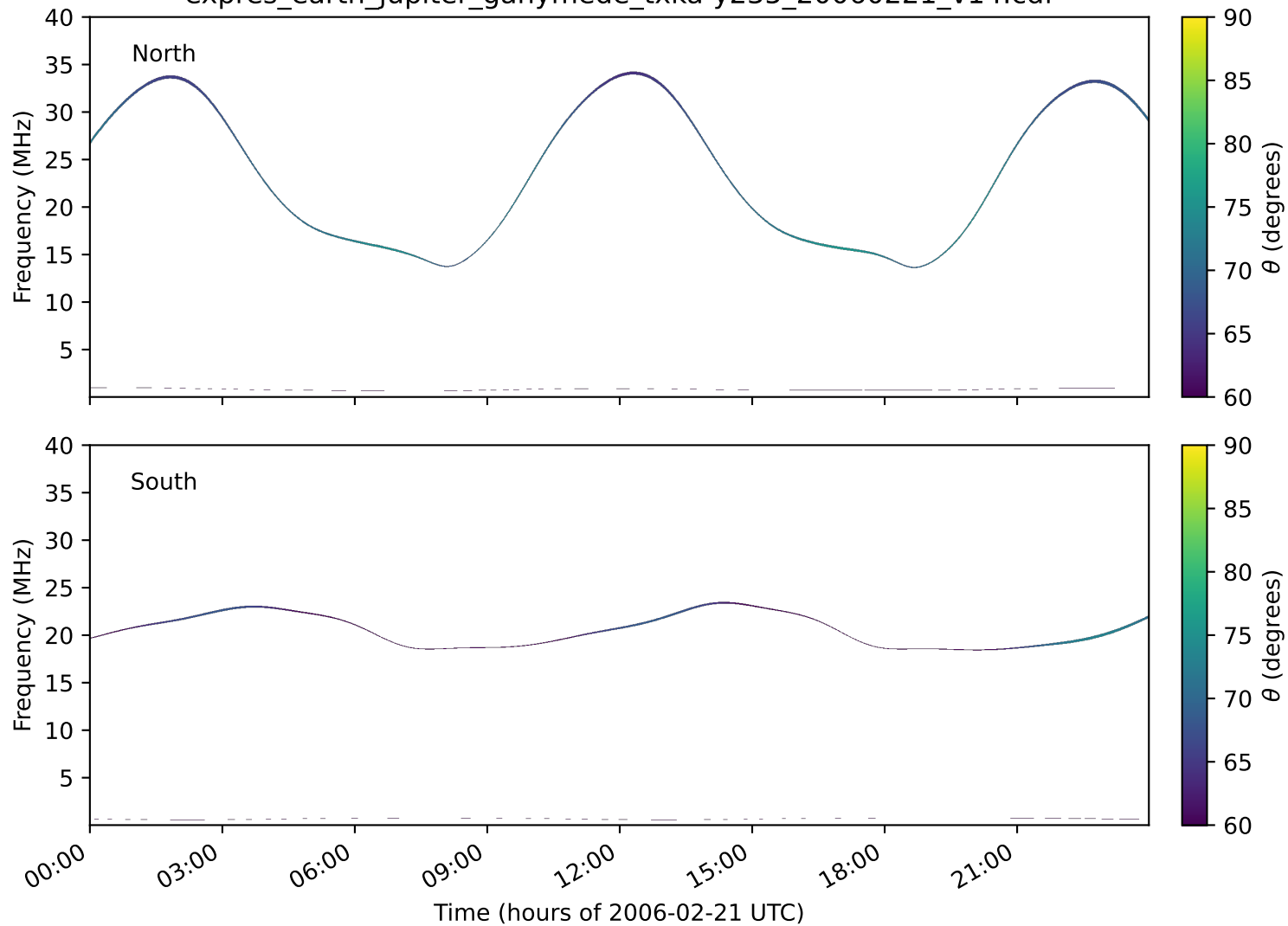
expres_earth_jupiter_ganymede_txka-y235_20060221_v14.cdf
