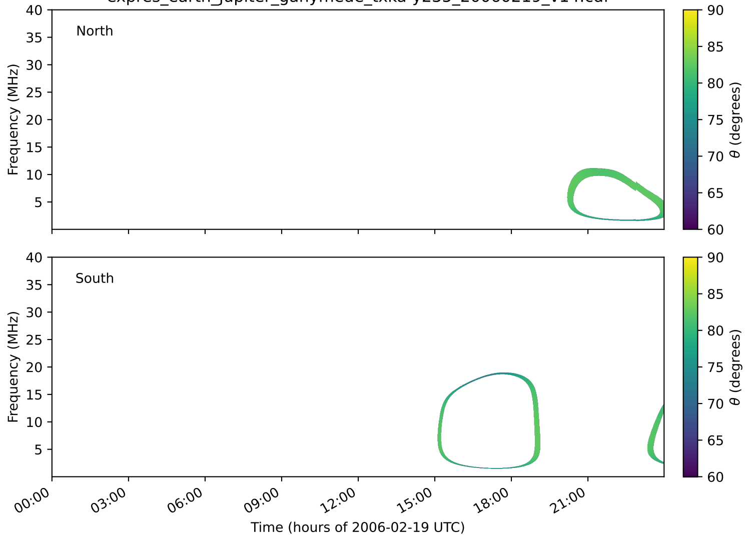
expres_earth_jupiter_ganymede_txka-y235_20060219_v14.cdf
