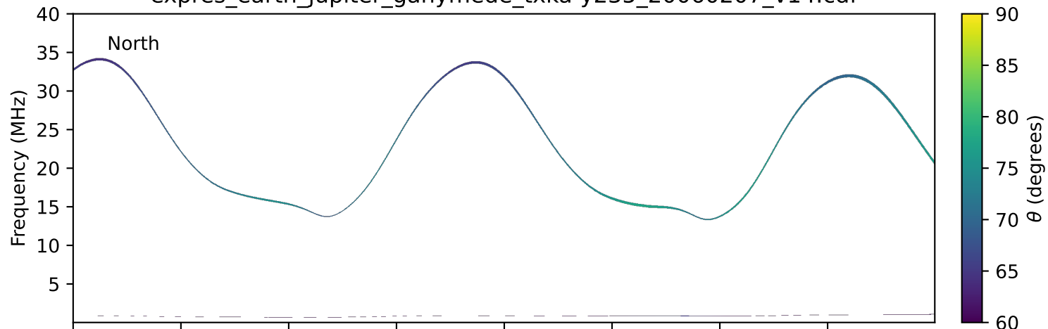
expres_earth_jupiter_ganymede_txka-y235_20060207_v14.cdf
