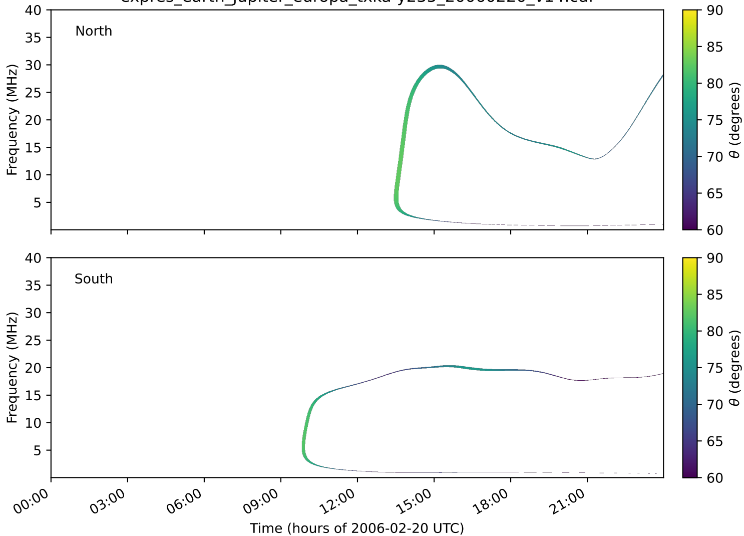
expres_earth_jupiter_europa_txka-y235_20060220_v14.cdf
