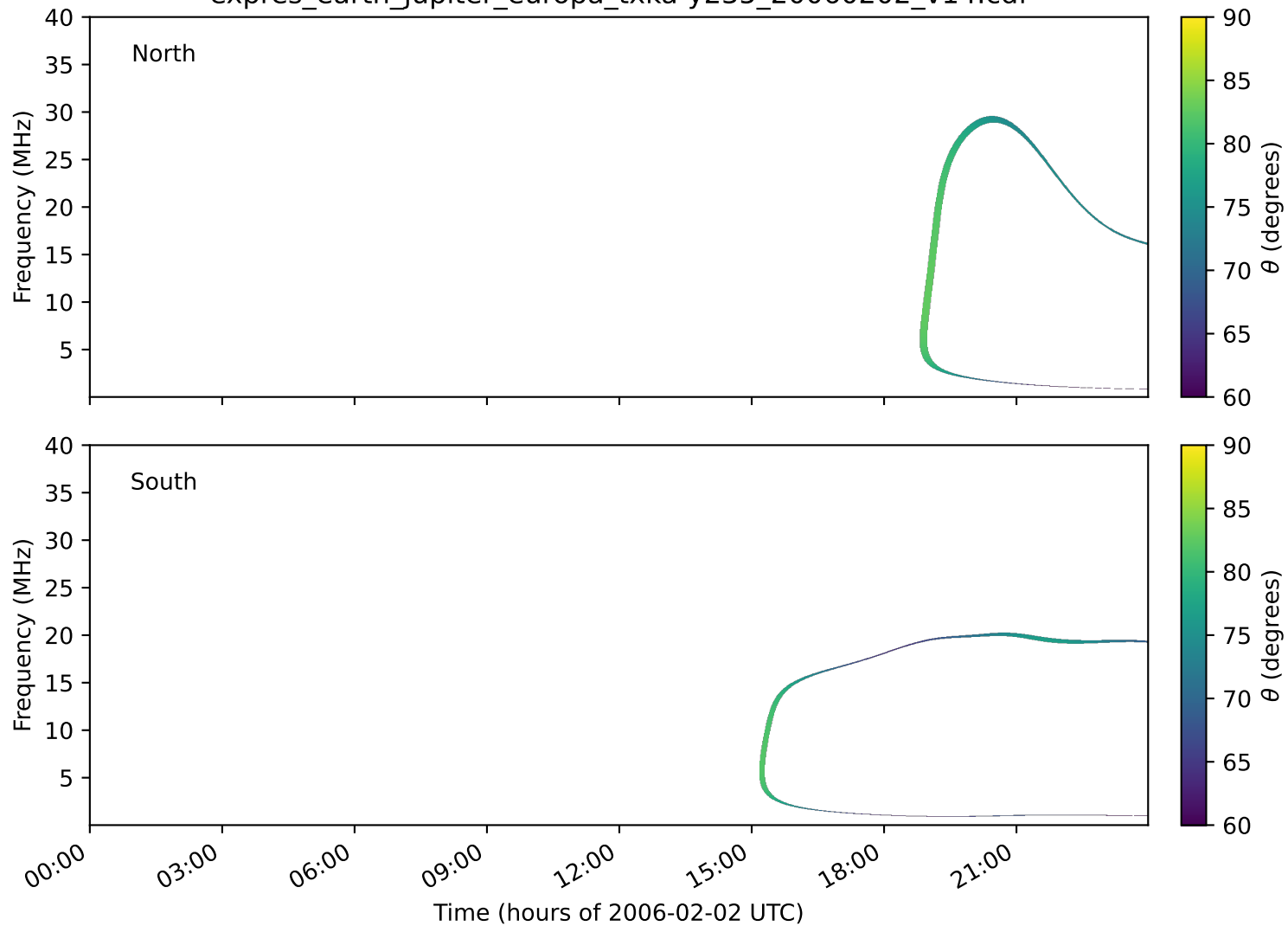
expres_earth_jupiter_europa_txka-y235_20060202_v14.cdf
