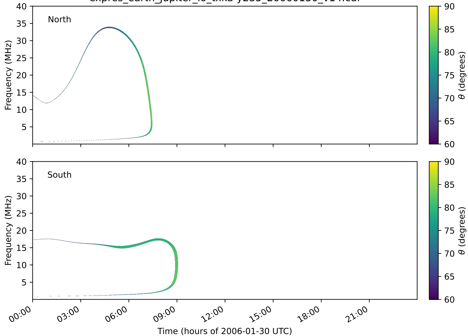
expres_earth_jupiter_io_txka-y235_20060130_v14.cdf
