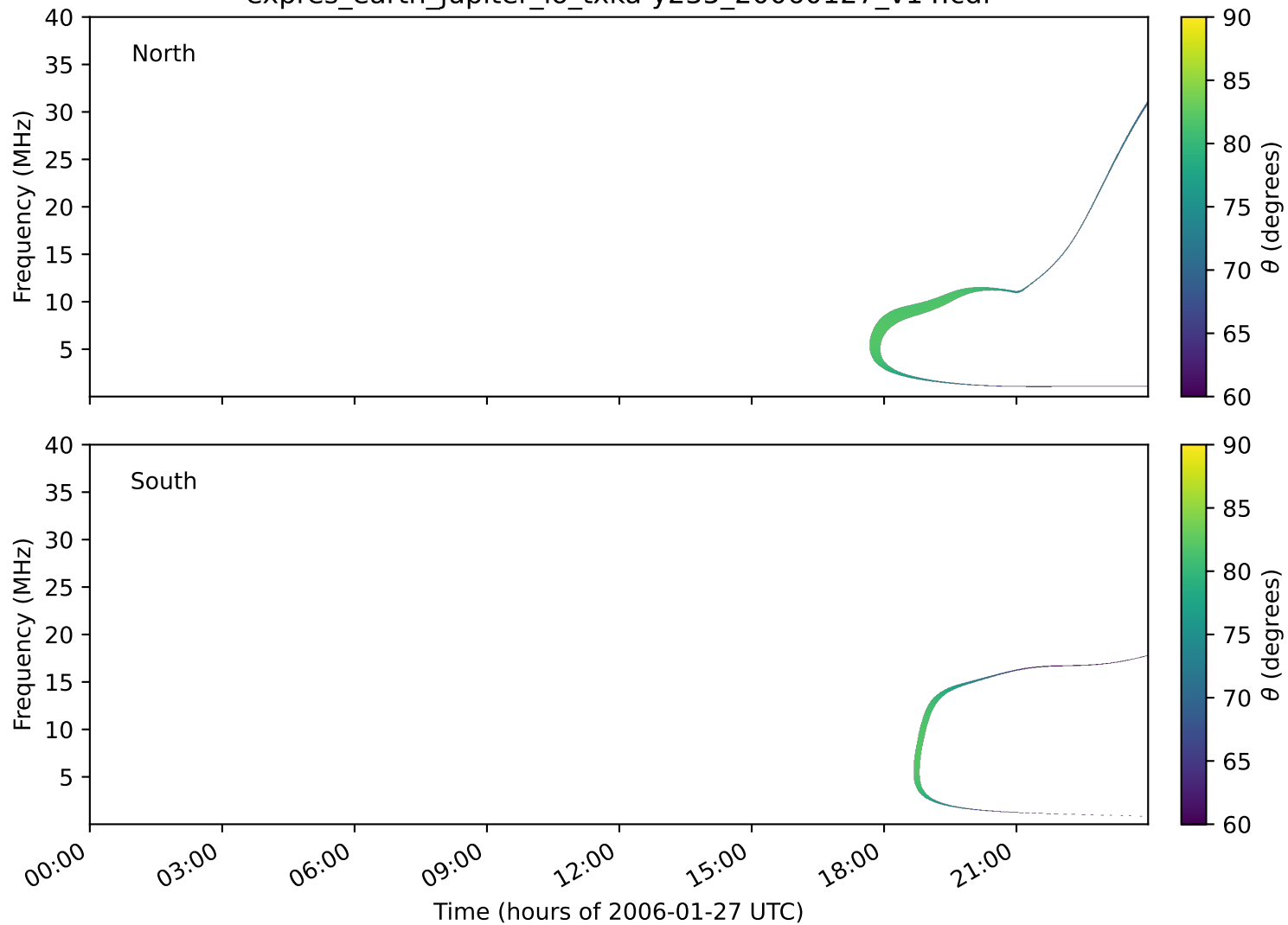
expres_earth_jupiter_io_txka-y235_20060127_v14.cdf
