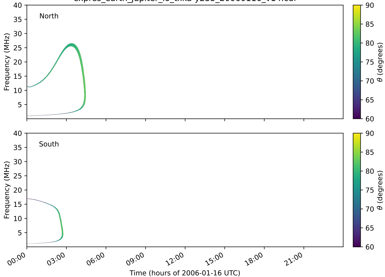
expres_earth_jupiter_io_txka-y235_20060116_v14.cdf
