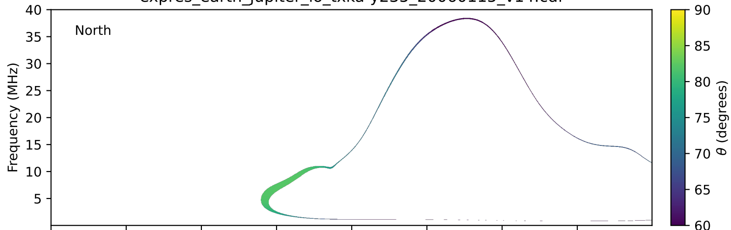
expres_earth_jupiter_io_txka-y235_20060115_v14.cdf
