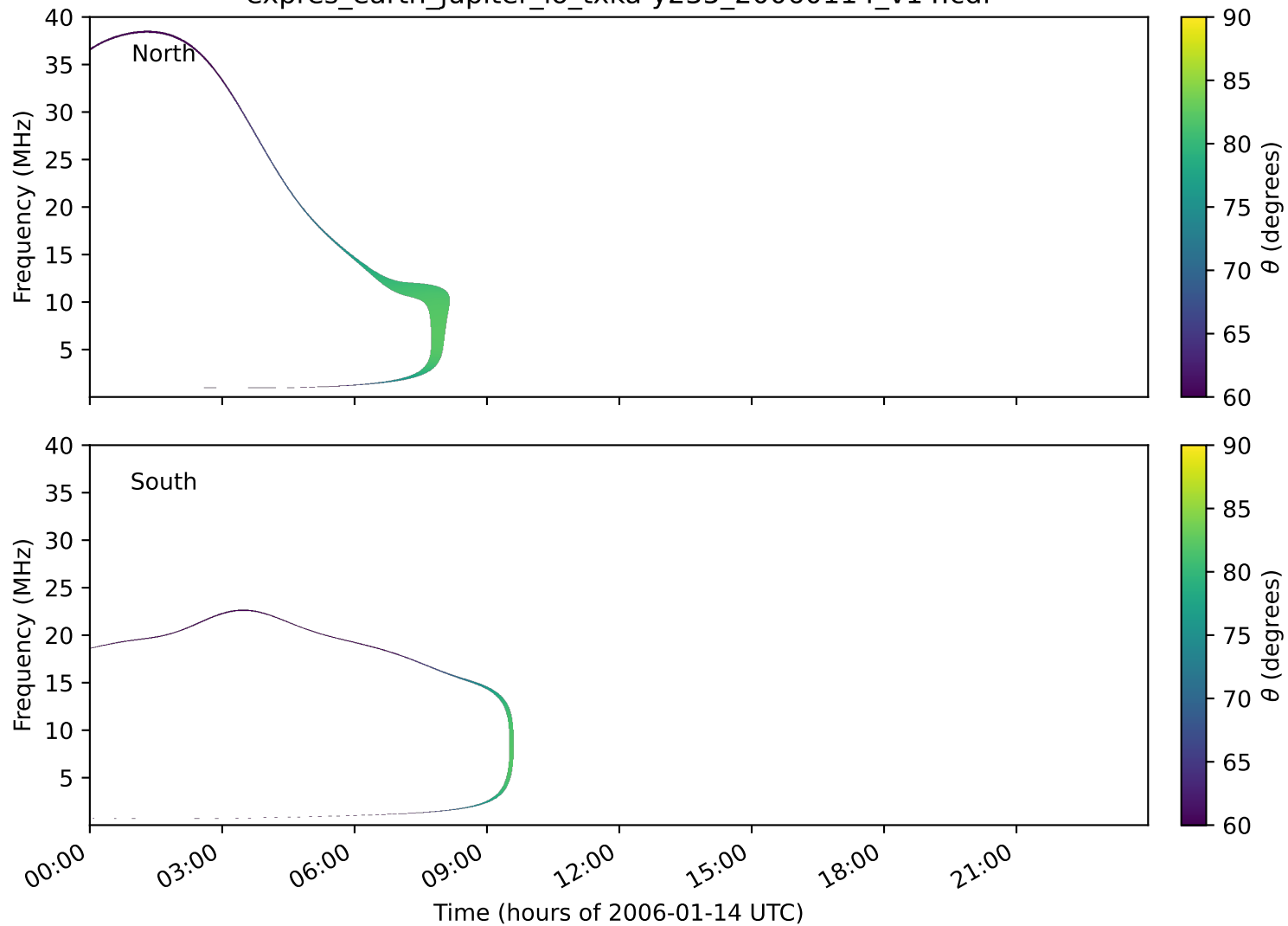
expres_earth_jupiter_io_txka-y235_20060114_v14.cdf
