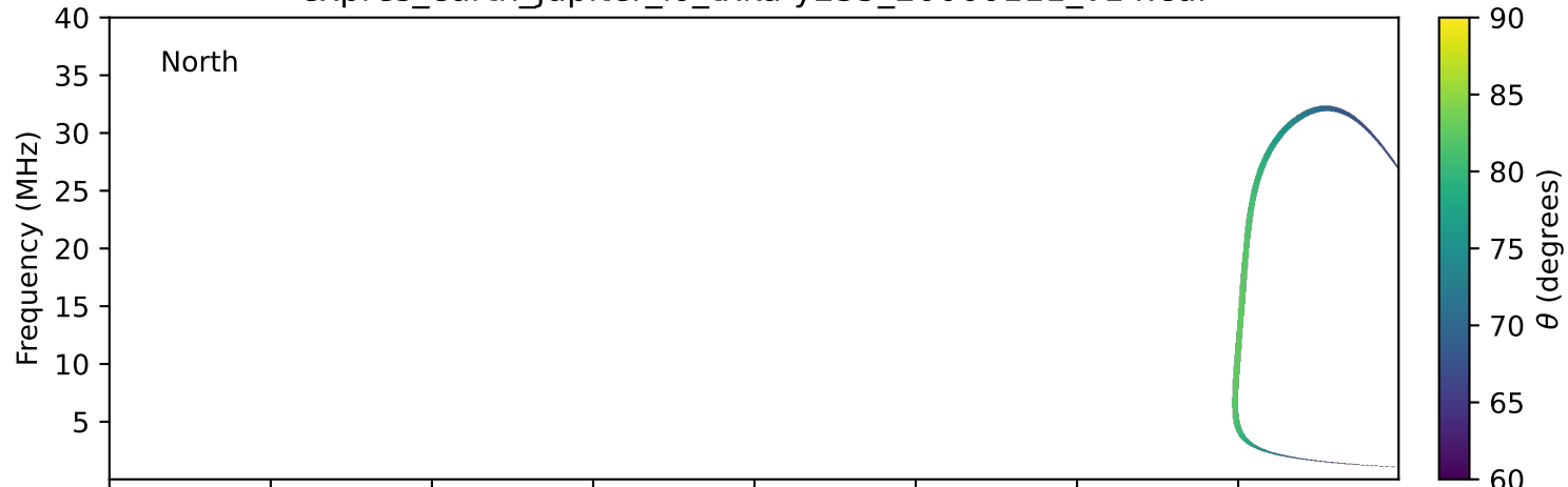
expres_earth_jupiter_io_txka-y235_20060111_v14.cdf
