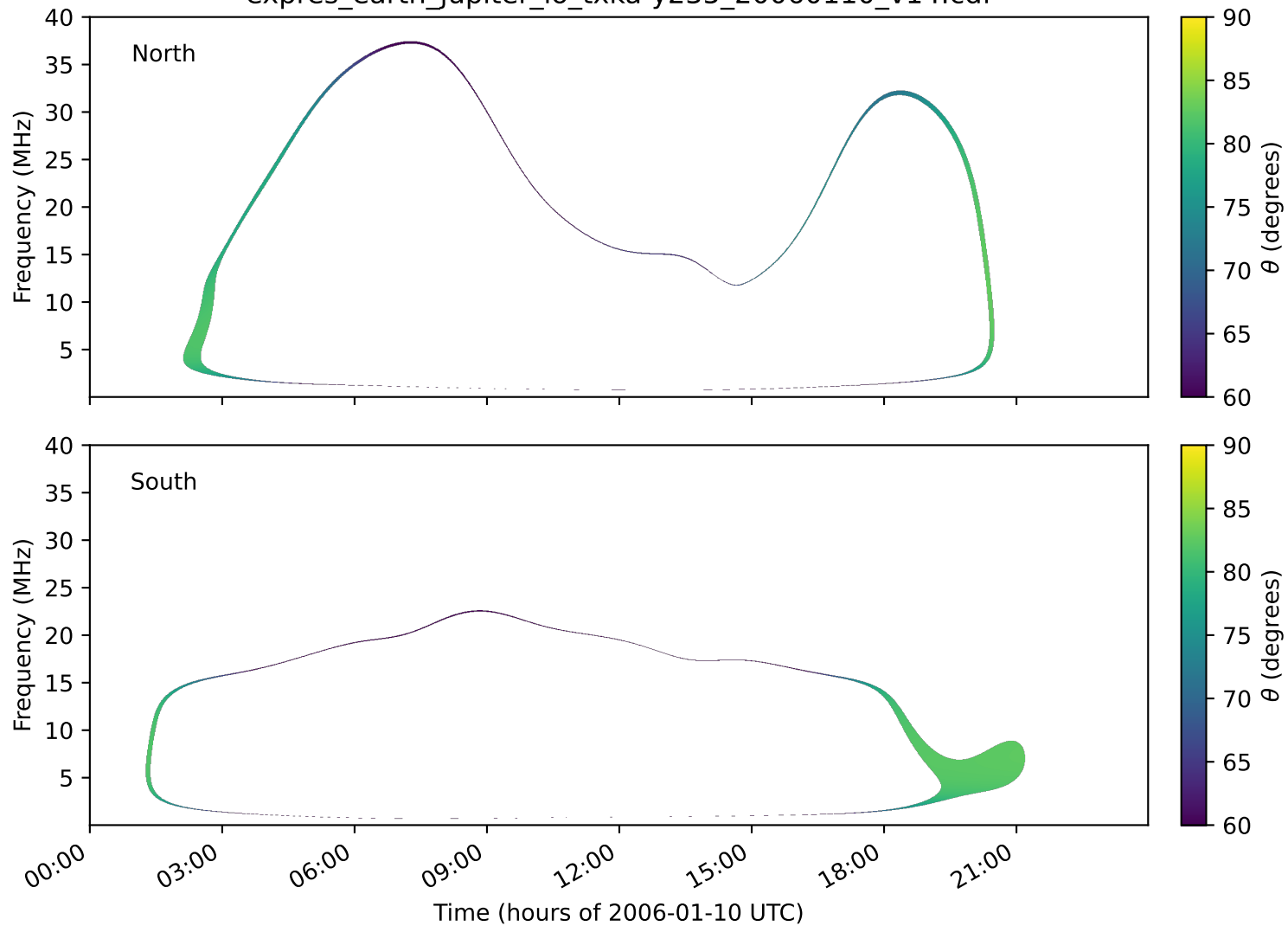
expres_earth_jupiter_io_txka-y235_20060110_v14.cdf
