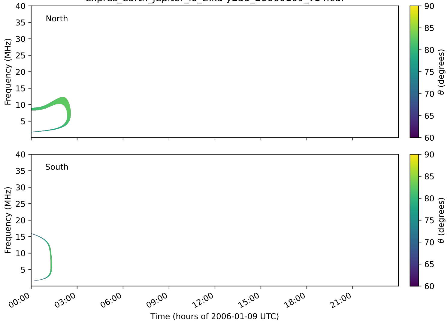
expres_earth_jupiter_io_txka-y235_20060109_v14.cdf
