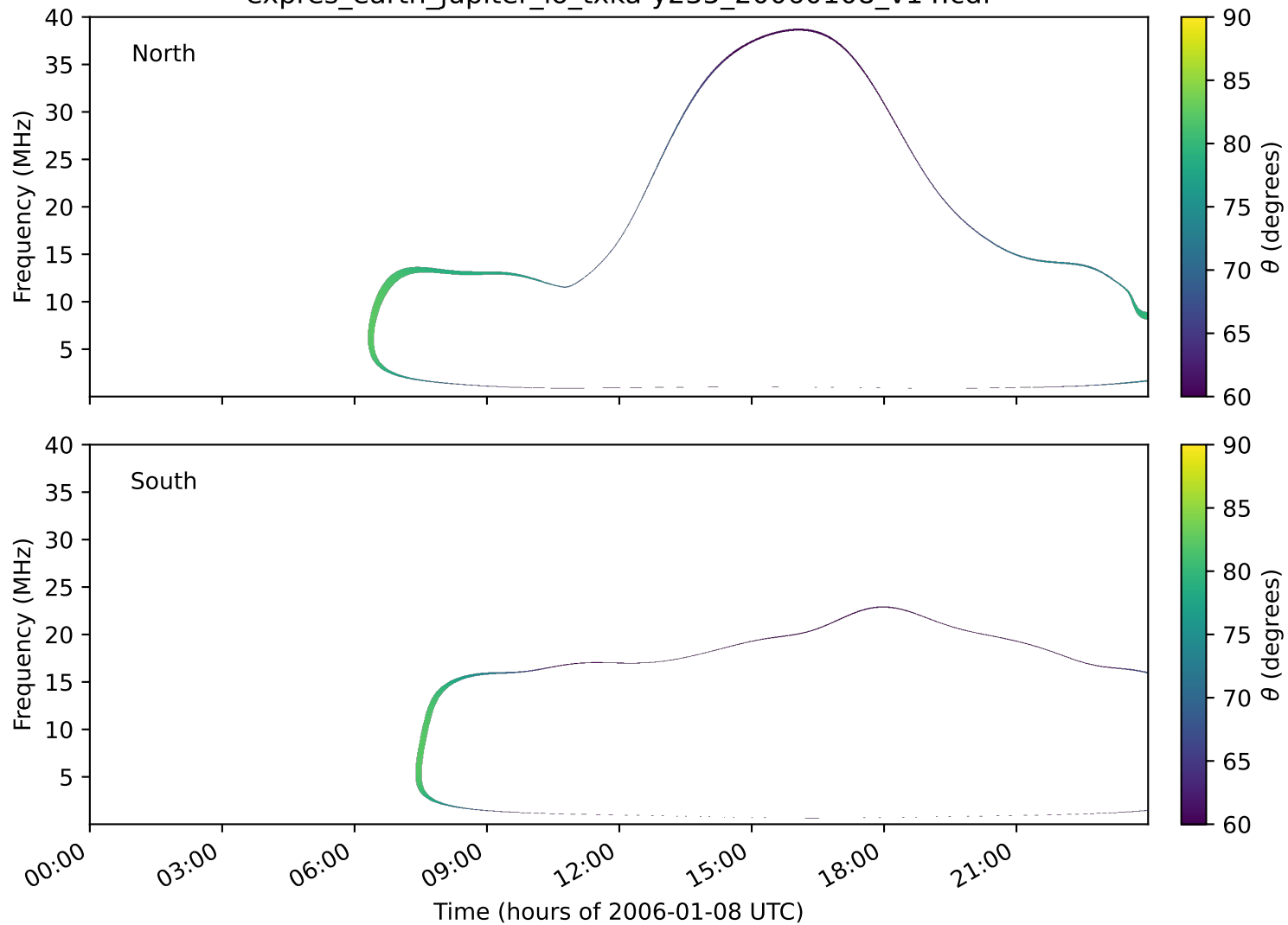
expres_earth_jupiter_io_txka-y235_20060108_v14.cdf
