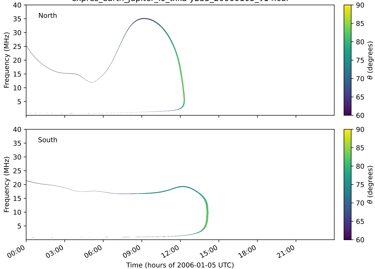
expres_earth_jupiter_io_txka-y235_20060105_v14.cdf
