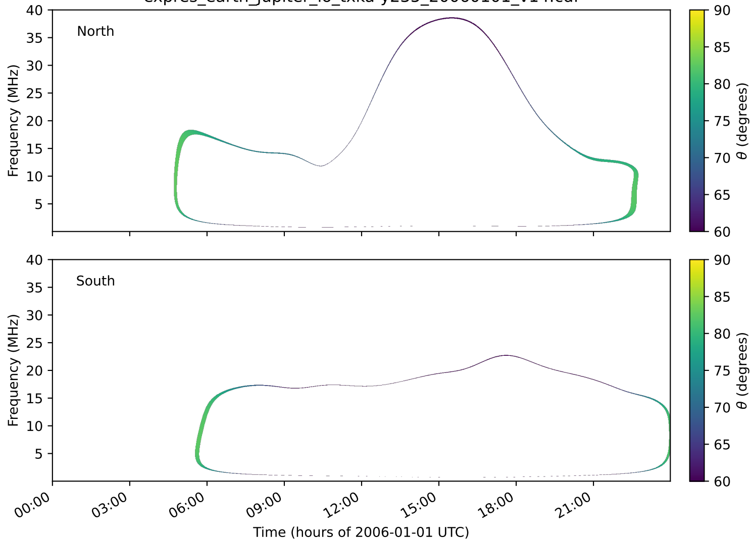
expres_earth_jupiter_io_txka-y235_20060101_v14.cdf
