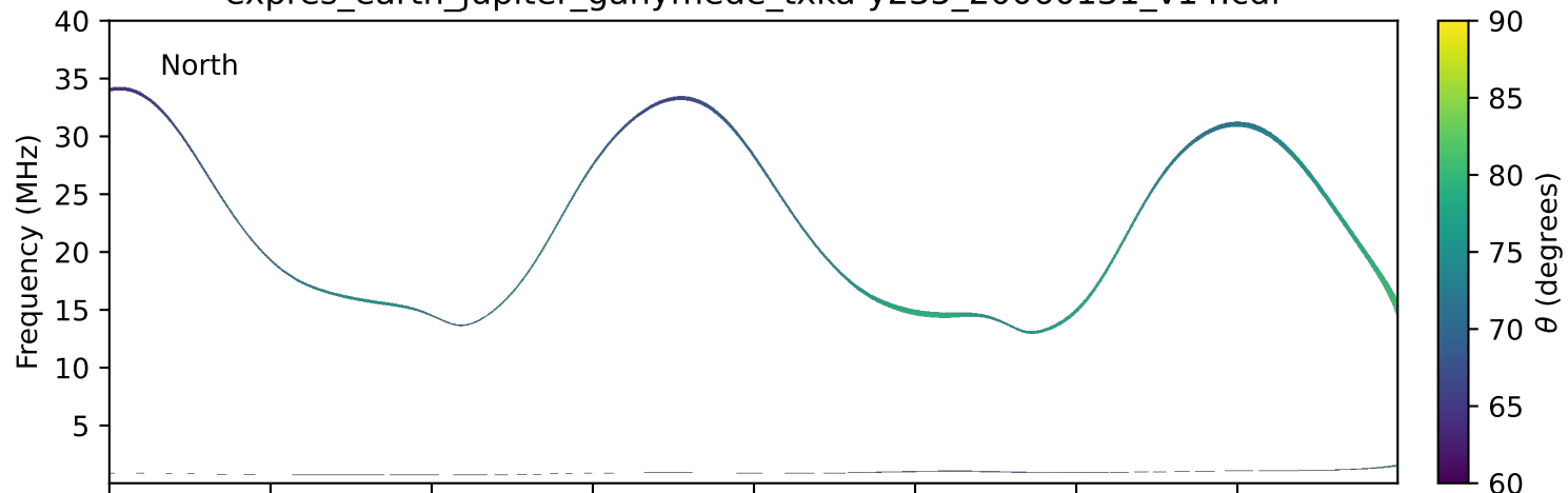
expres_earth_jupiter_ganymede_txka-y235_20060131_v14.cdf
