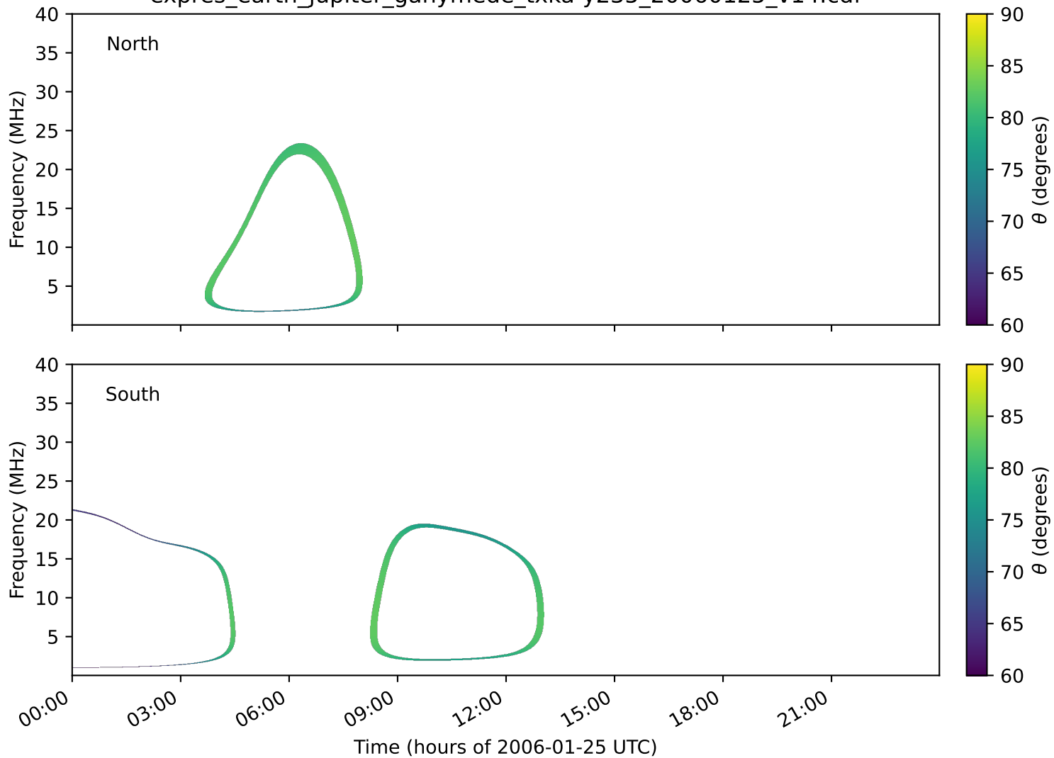
expres_earth_jupiter_ganymede_txka-y235_20060125_v14.cdf
